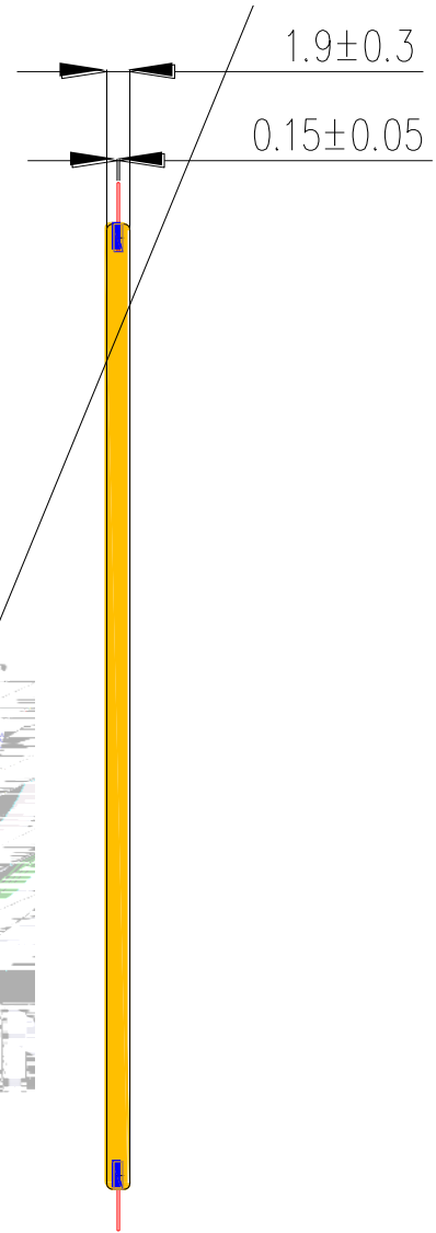
Fig.1-2 Bottom view
