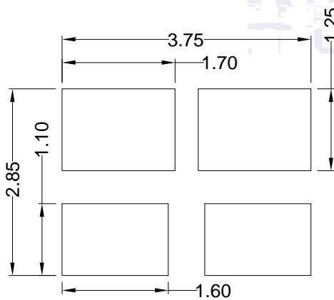
Fig.1-5 Soldering Patterns
