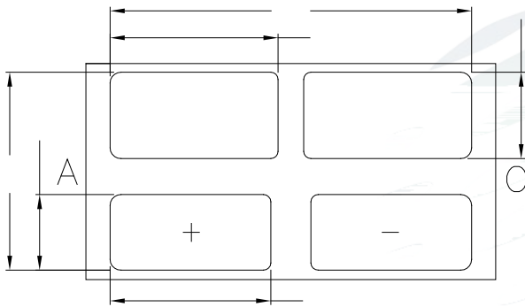
Fig.1-3 Bottom View
