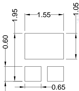
Fig.1-5 Soldering Patterns
