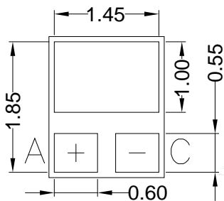
Fig.1-3 Bottom View
