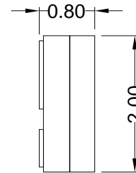
Fig.1-2 Side View
