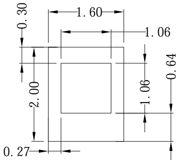
Fig.1-1 Top View
