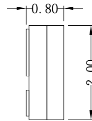
Fig.1-2 Side View
