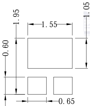
Fig.1-5 Soldering Patterns
