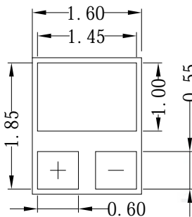
Fig.1-3 Bottom View
