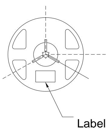
Fig.2-2Reel Dimension 卷盘
