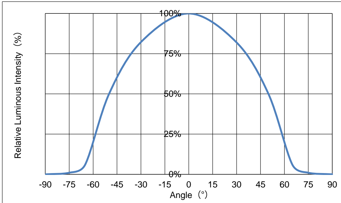
Fig 1-10 Radiation
